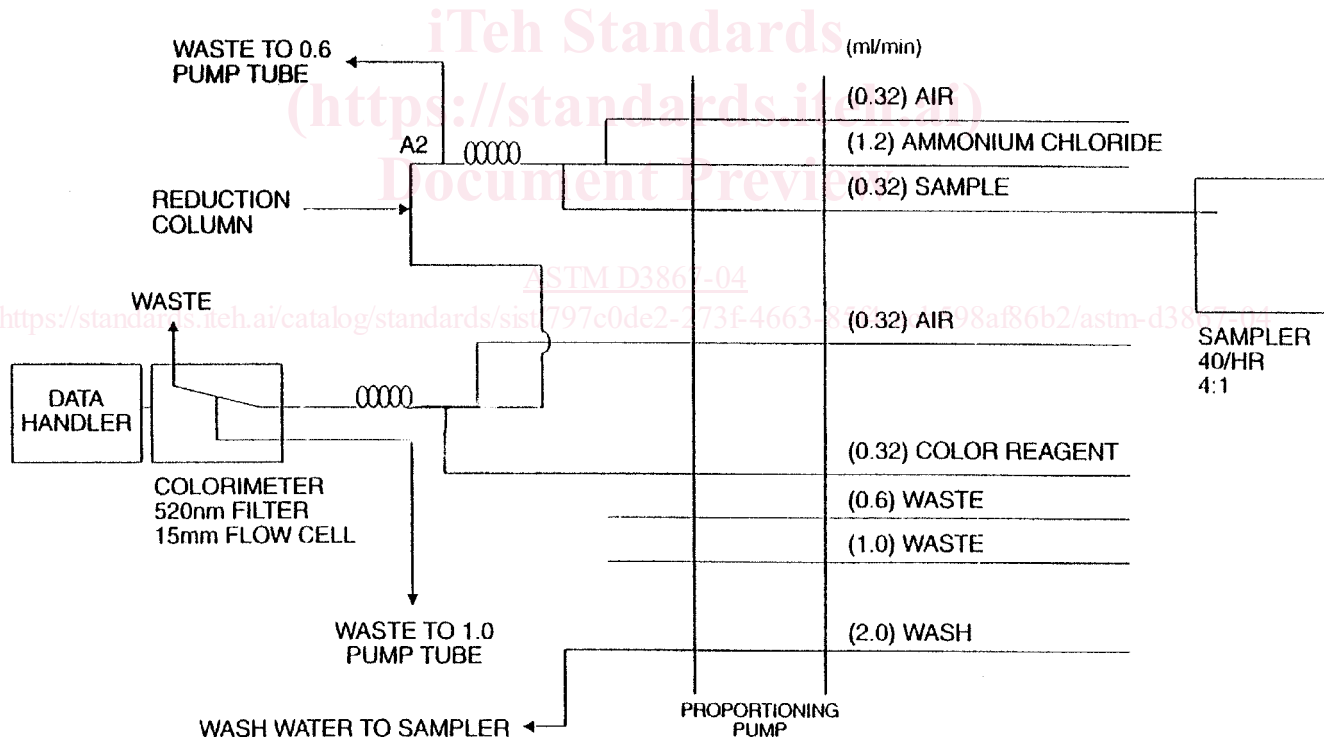
FIG. 2 Nitrite-Nitrate Cartridge
