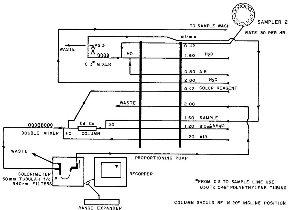
FIG. 1 Nitrite-Nitrate Manifold
