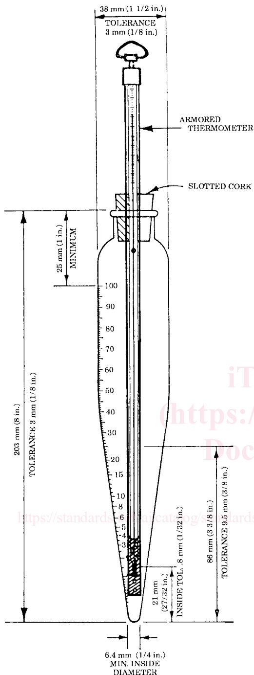
NOTE 1—For graduation tolerances see Table 1. FIG. 1 Weathering Tube
