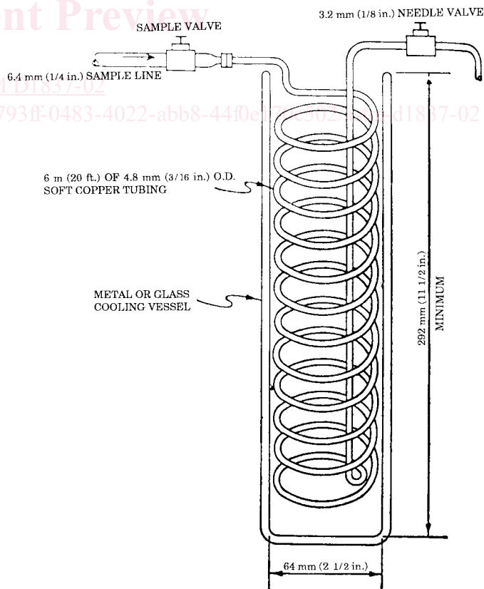
NOTE 1—The coils in the drawing are extended for clarity. FIG. 2 Precooling Equipment
