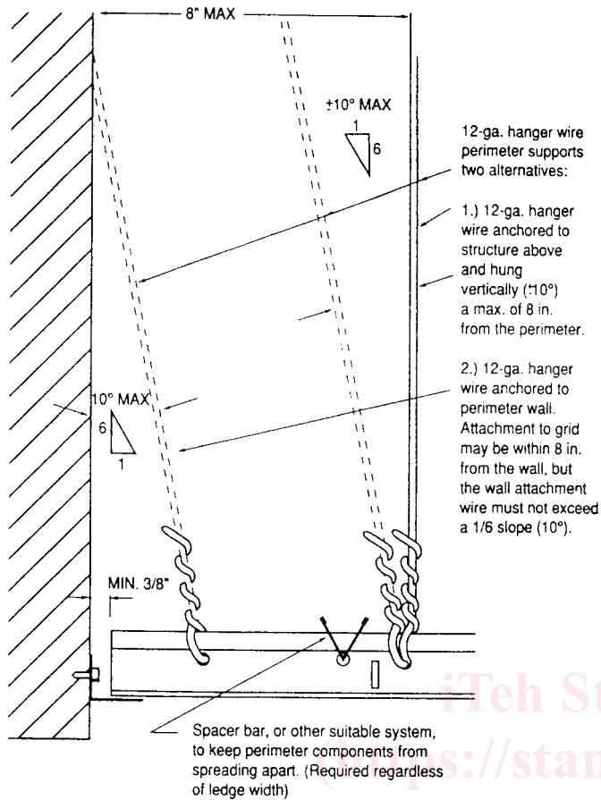
FIG. 3 Light to Moderate Treatment of Cross Runners and Main Runners at Terminal Ends When Support Ledge of Perimeter Closure is Less Than Minimum 7/8 in.
