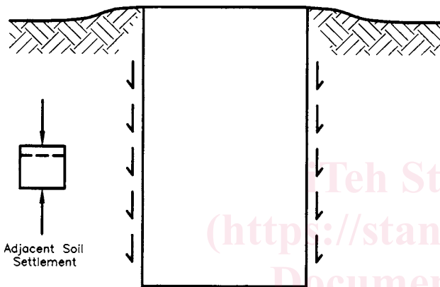
FIG. 3 Downdrag Force Acting on Manhole (Assumed for Design)
