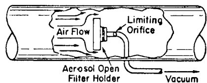
FIG. 5 Faulty Sample from a Rapid-Ducted Gas Stream
