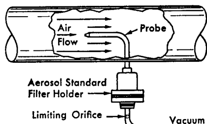
FIG. 4 Isokinetic Sampling from a Duct
