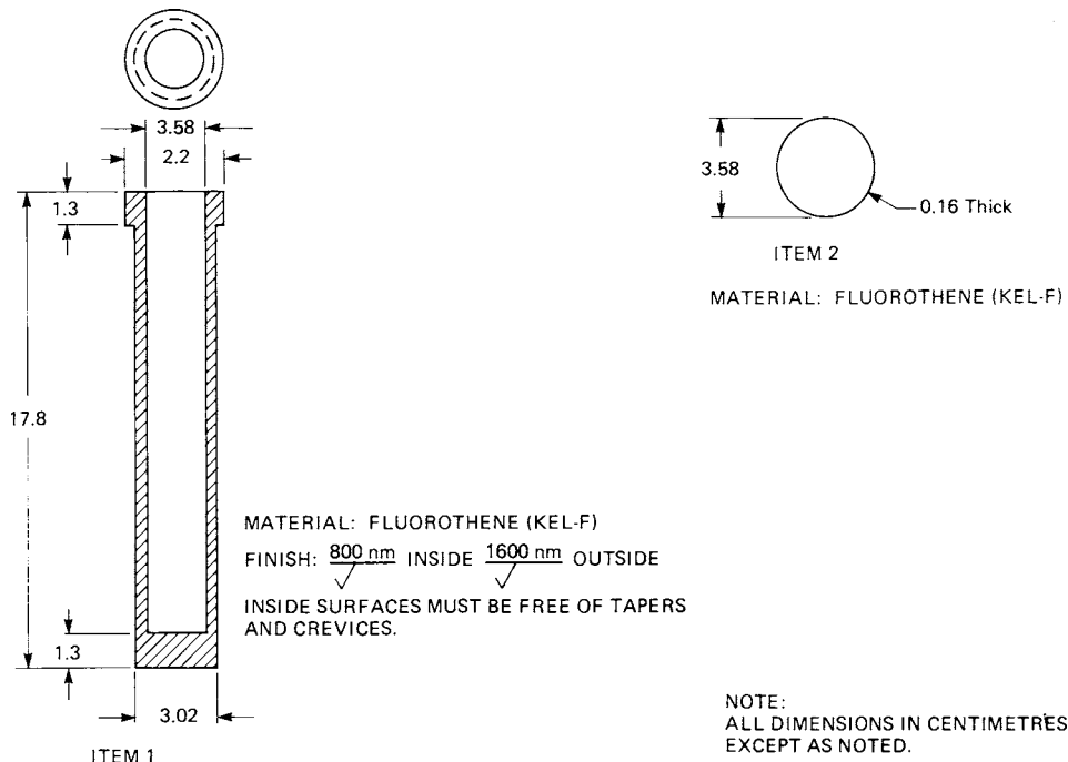
FIG. 4 polychlorotrifluoroethylene Knockout Cylinder
