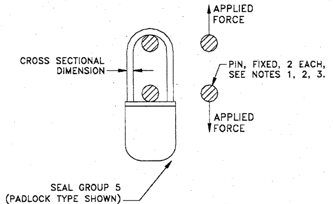
FIG. 4 Schematic Drawings of Pull (Tensile) Test Fixture Requirements for Group 5
