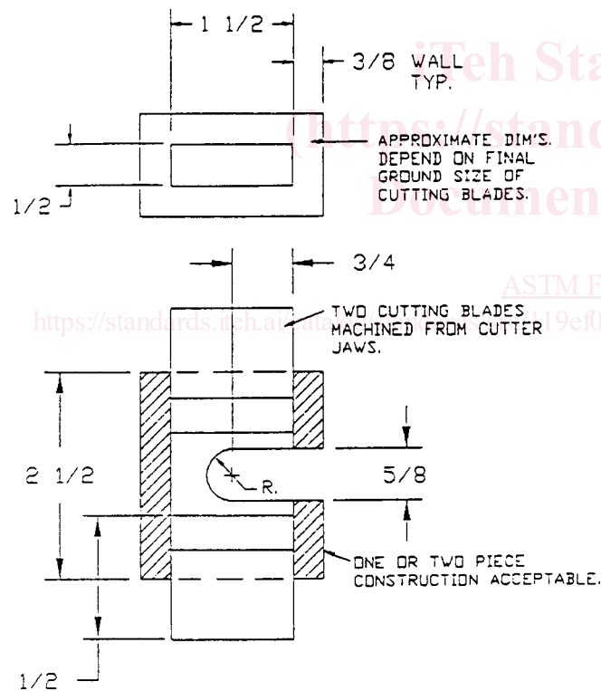
FIG. 5 Schematic Drawings of Possible Pull (Tensile) Test Fixture Configurations
