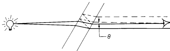
FIG. 1 Drawing of Light Ray Paths that Cause an Apparent Angular Separation ( \theta ) Between the Primary Image and the Secondary Image
