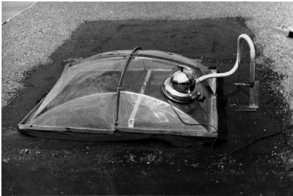
FIG. 1 View of Chamber over Roof Test Area During Test
