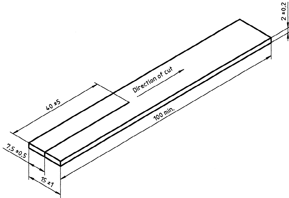
Figure 1 — Trouser test piece die iTeh STANDARD PREVIEW (standards.iteh.ai)
