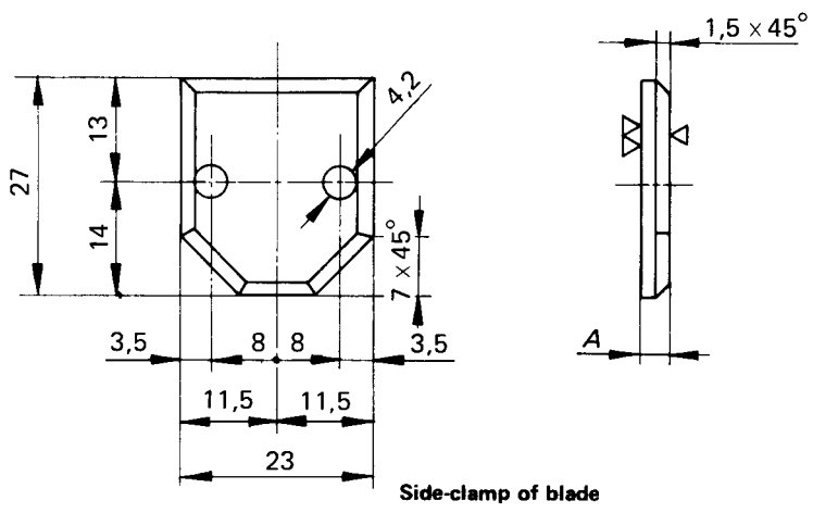
FIGURE 2 – Special tool, holding removable blades
