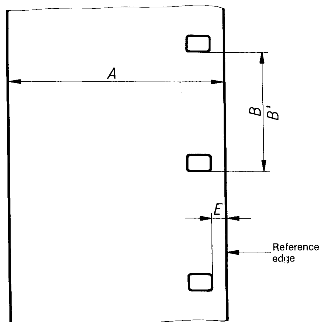
Figure 1 — Film with perforations along one edge (Type 1)
