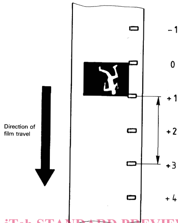
Figure A.1 — Standard image position reference (standards.iteh.ai)
