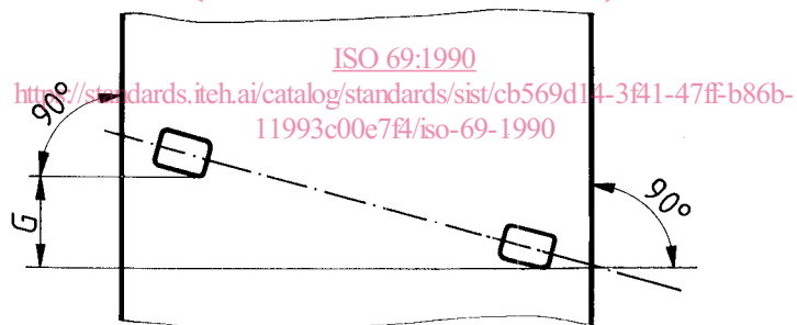
Figure 4 — Permissible alignment deviation of the rows of perforations (Type 2)
