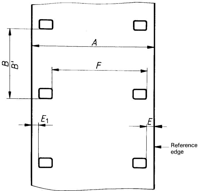
Figure 2 — Film with perforations along two edges (Type 2)
