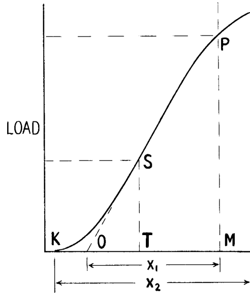
FIG. 1 b Compressive Strength (See 3.1.5 and Section 9)
