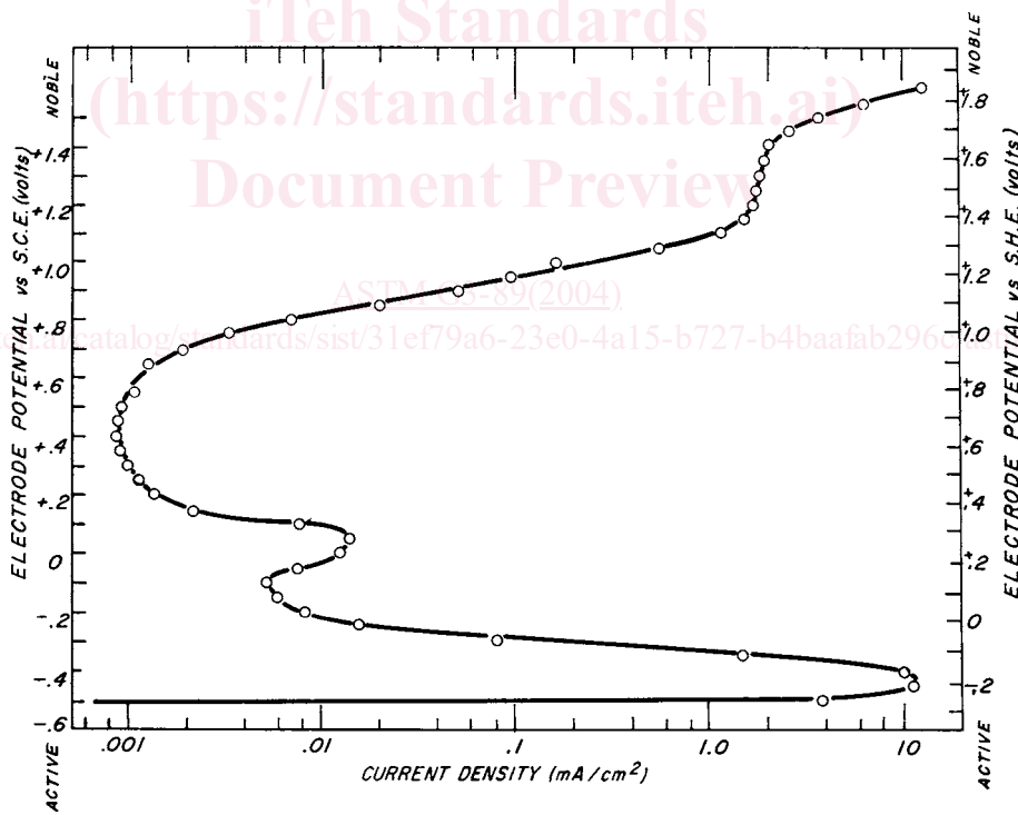
FIG. 5 Typical Potentiostatic Anodic Polarization Plot for Type 430 Stainless Steel in 1.0 N H 2 SO 4
