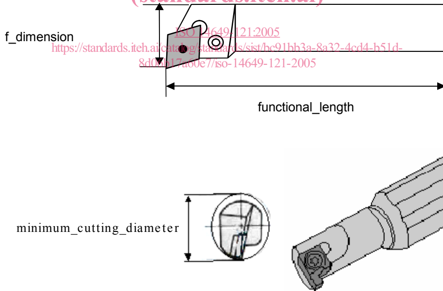
Figure 1 : Turning machine tool.
