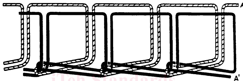
DIRECTION OF SUCCESSIVE STITCH FORMATION
