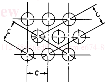
FIG. 1 Arrangement of Round Apertures.
