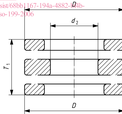
Figure 2 — Double-direction bearings
