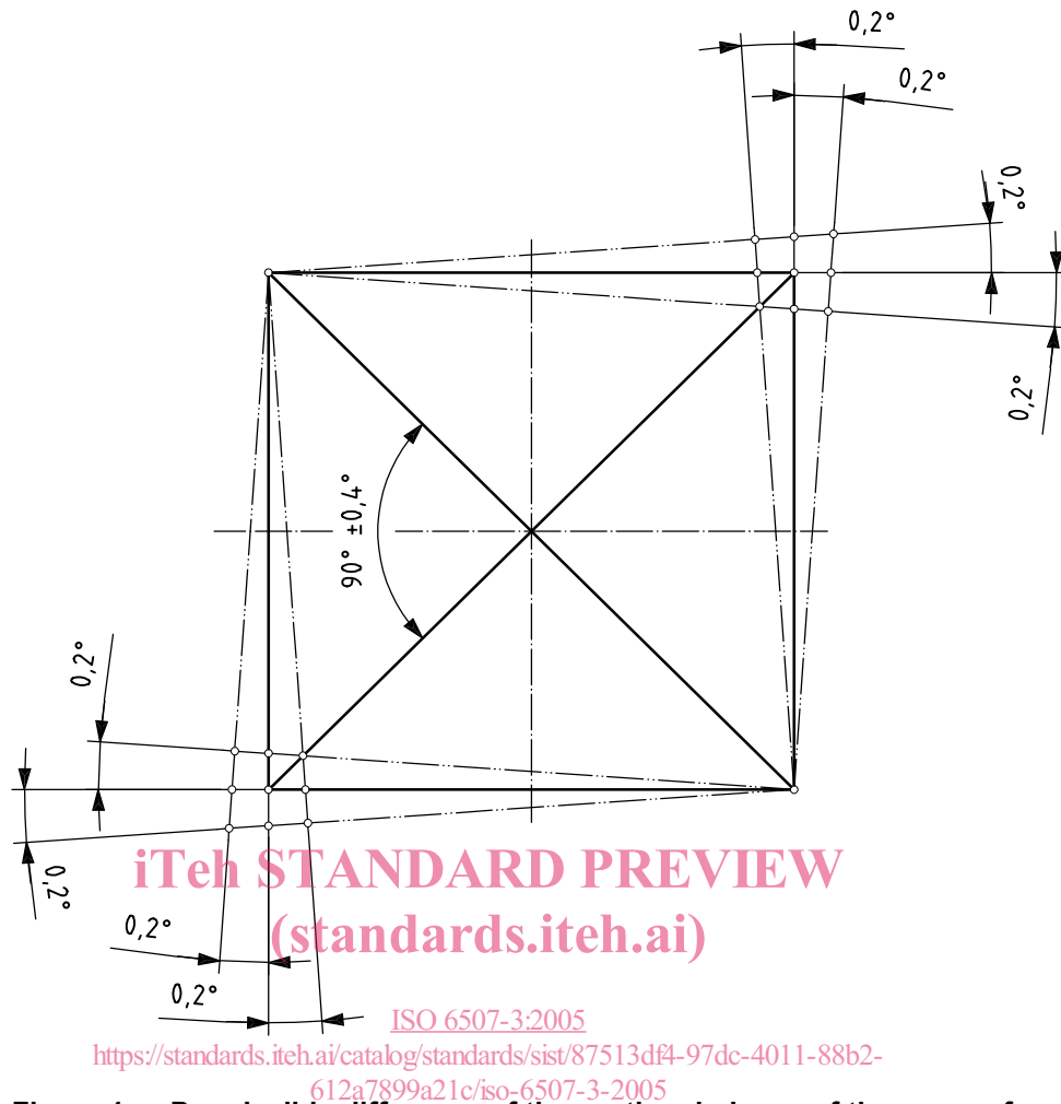
Figure 1 — Permissible difference of the sectional planes of the square form
