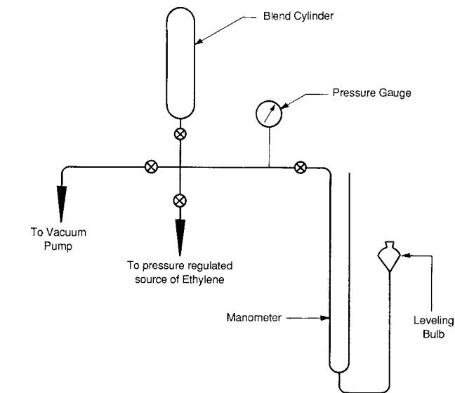
FIG. 2 Gas-Blending Manifold
