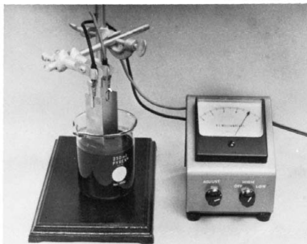
FIG. 2 Particle Charge Tester
