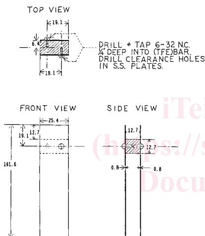
FIG. 4 Insulator
