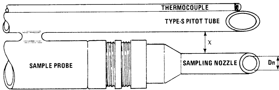
FIG. 7 Typical Pitobe Assembly
