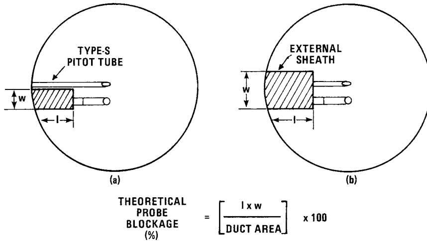
FIG. 5 Projected-Area Models for Typical Pitotube Assemblies
