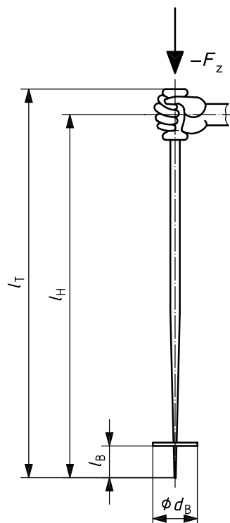
Figure 2 — Centre of rotation and dimensions (standards.iteh.ai)
