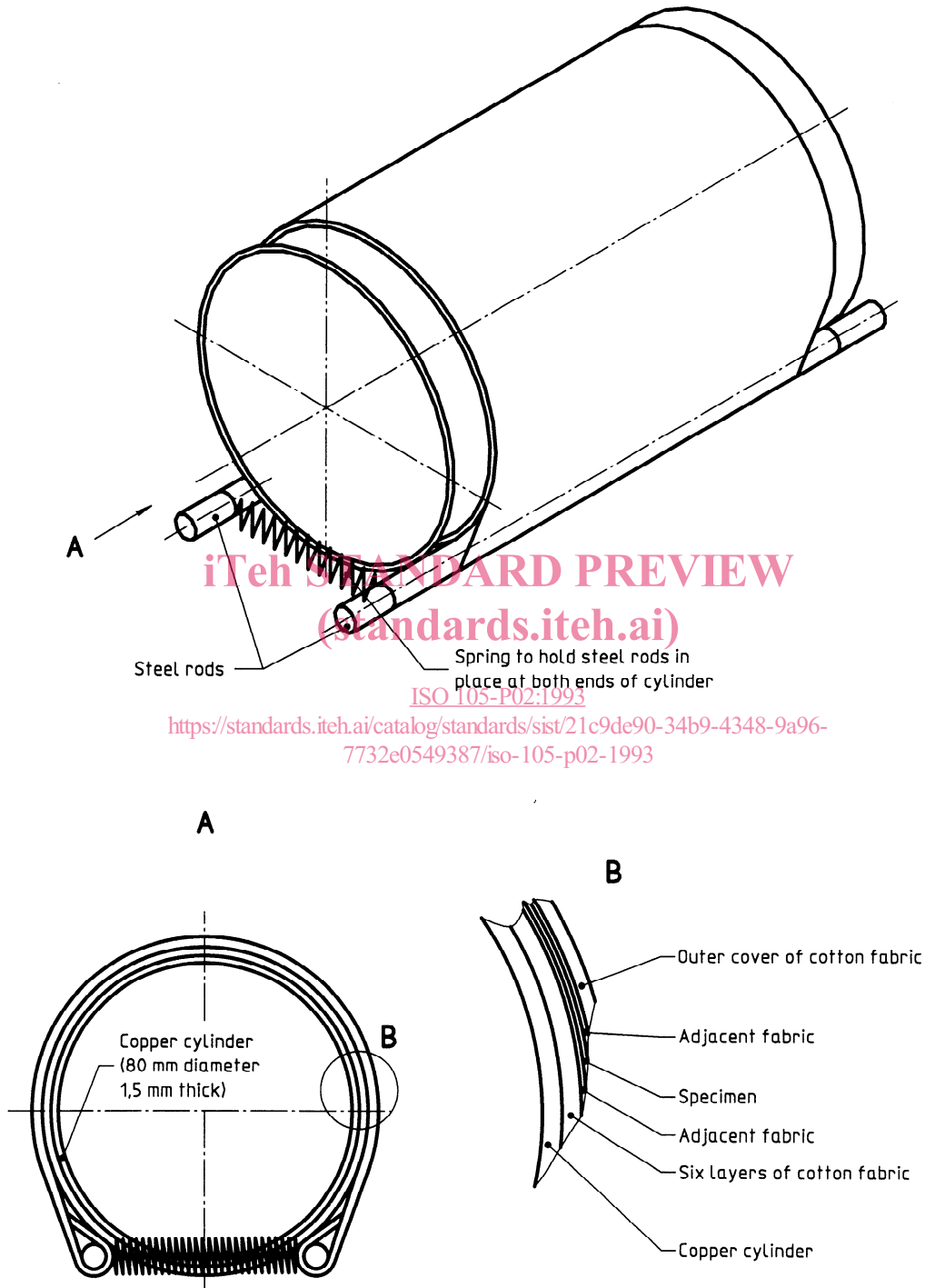
Figure 1 — Specimen holder
