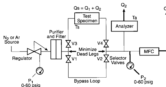
FIG. 1 Test Schematic
