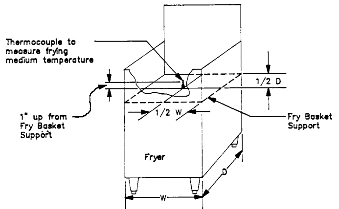
FIG. 2 Thermocouple Placement
