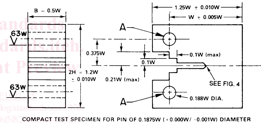
FIG. 1 Recommended Compact Specimen Designs
