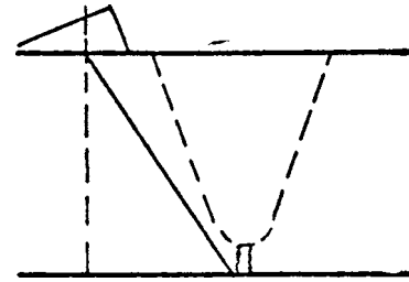
FIG. 12 Incomplete Penetration
