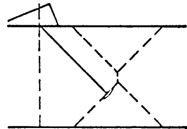
FIG. 13 Incomplete Fusion
