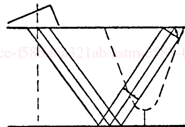
FIG. 15 Cracks
