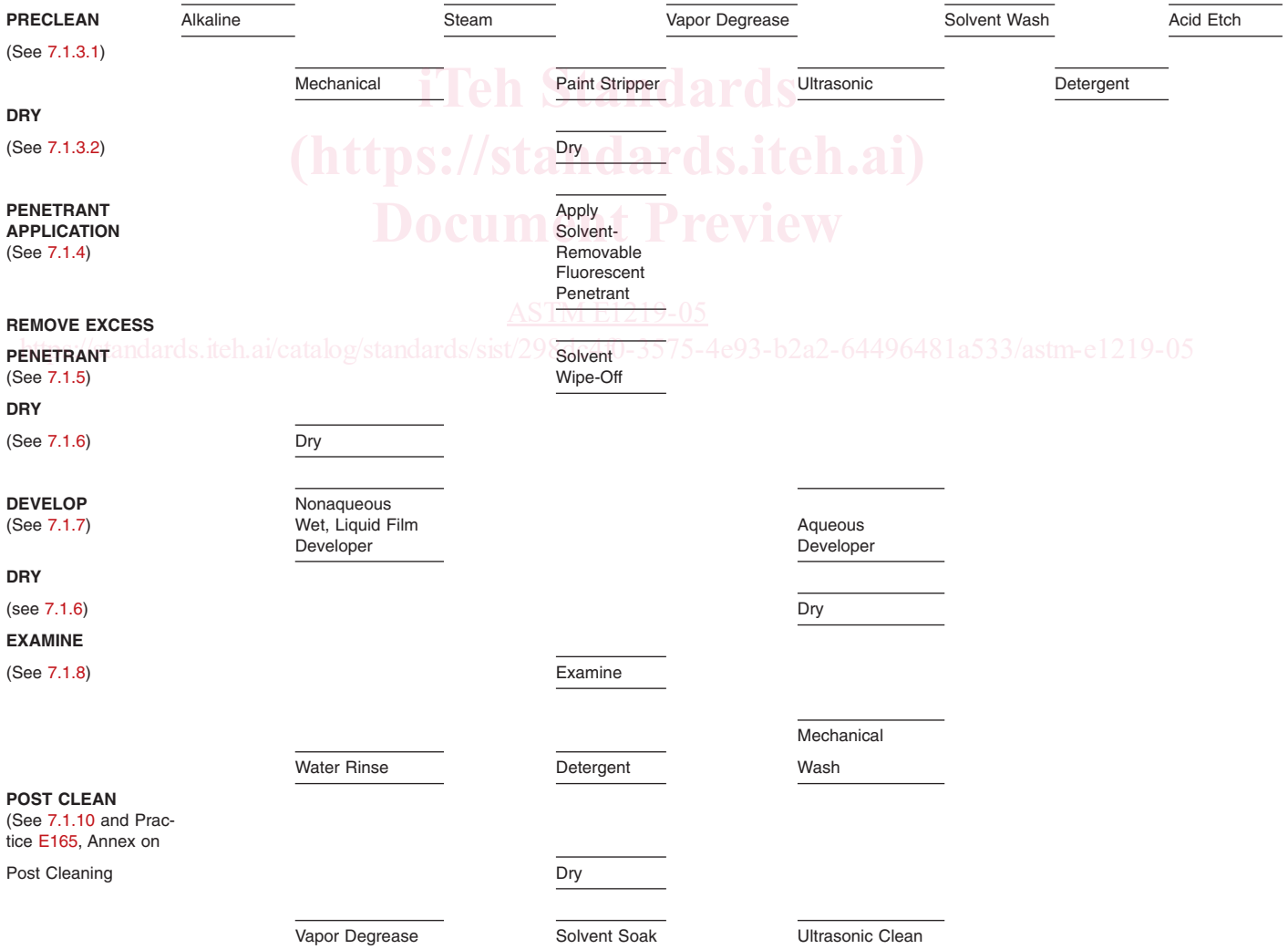
FIG. 1 Solvent-Removable Fluorescent Penetrant Examination General Procedure Flowsheet
