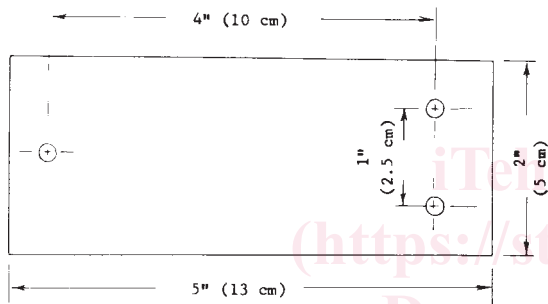
FIG. 4 Test Specimen
