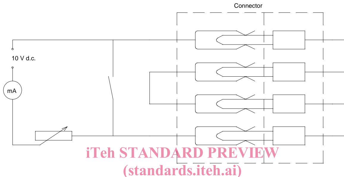
Figure 1 – Test circuit
