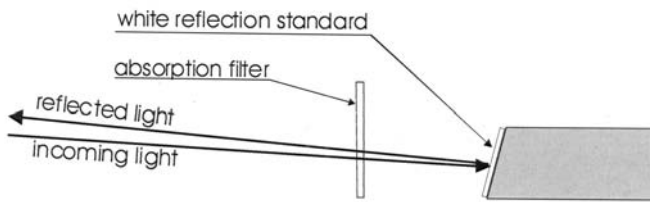
FIG. 1 White Reflection Standard and Absorption Filter for Testing Spectral Match
