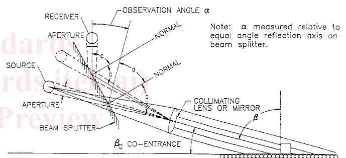
FIG. 2c Angles and apertures for portable retroreflector with collimating and beam splitter design
