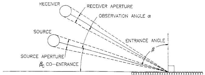
FIG. 2a Angles and apertures for non-collimating portable retroreflector
