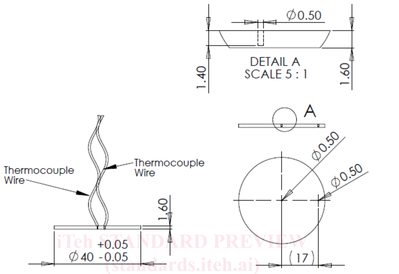
a) calorimeter assembly with mounting pins omitted for clarity
