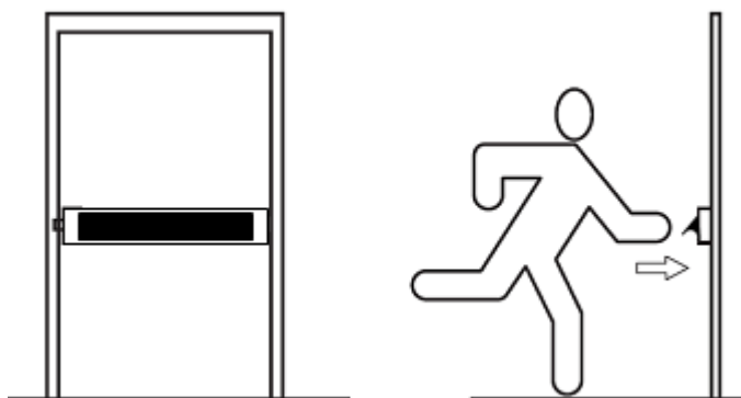
Figure 4 — Panic exit device with type C bar operation (Pivot touch-bar)
