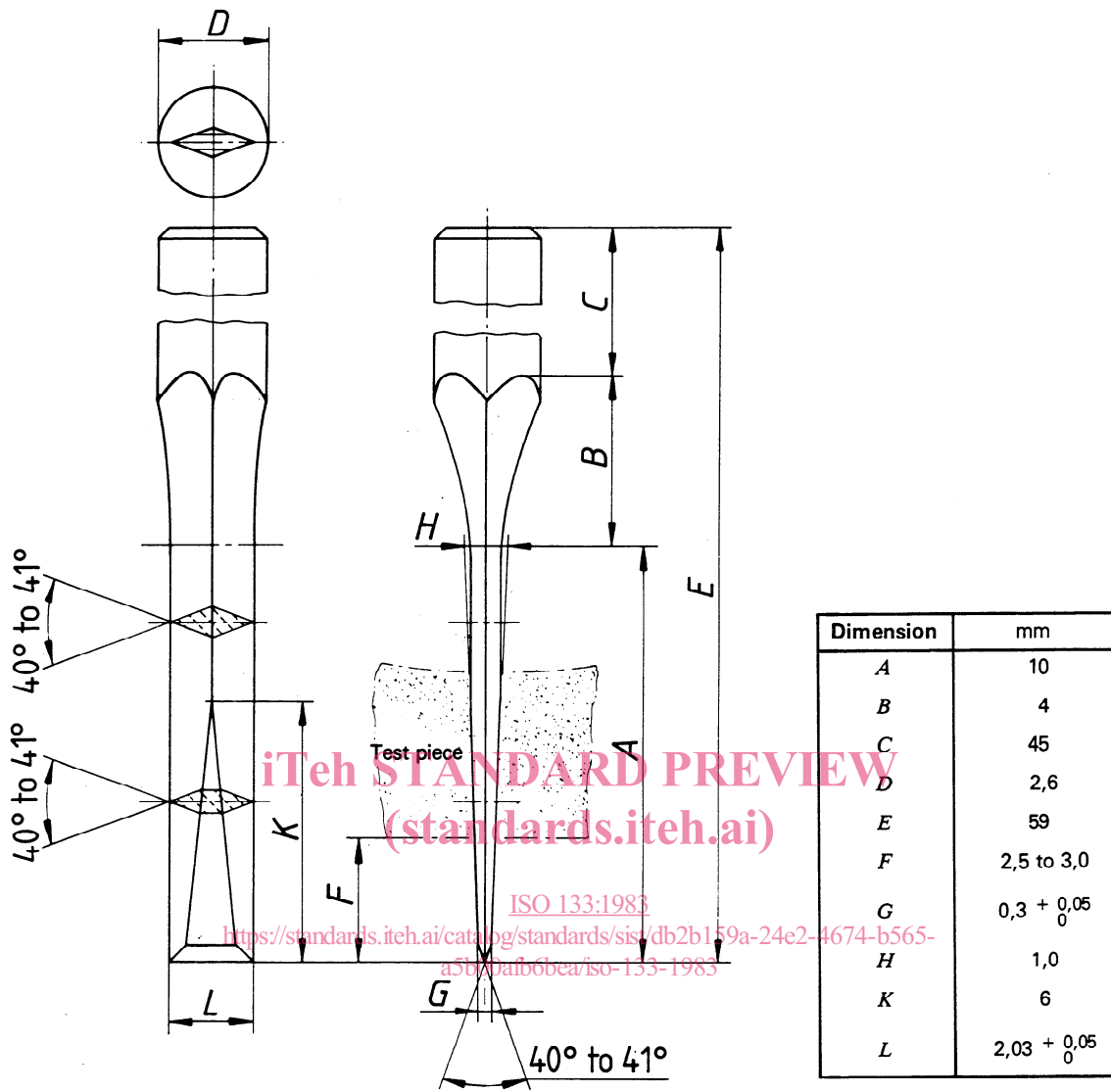
Figure 3 — Piercing tool
