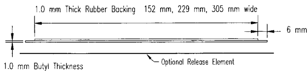
FIG. 3 Sealing Band Type III (Not to Scale)
