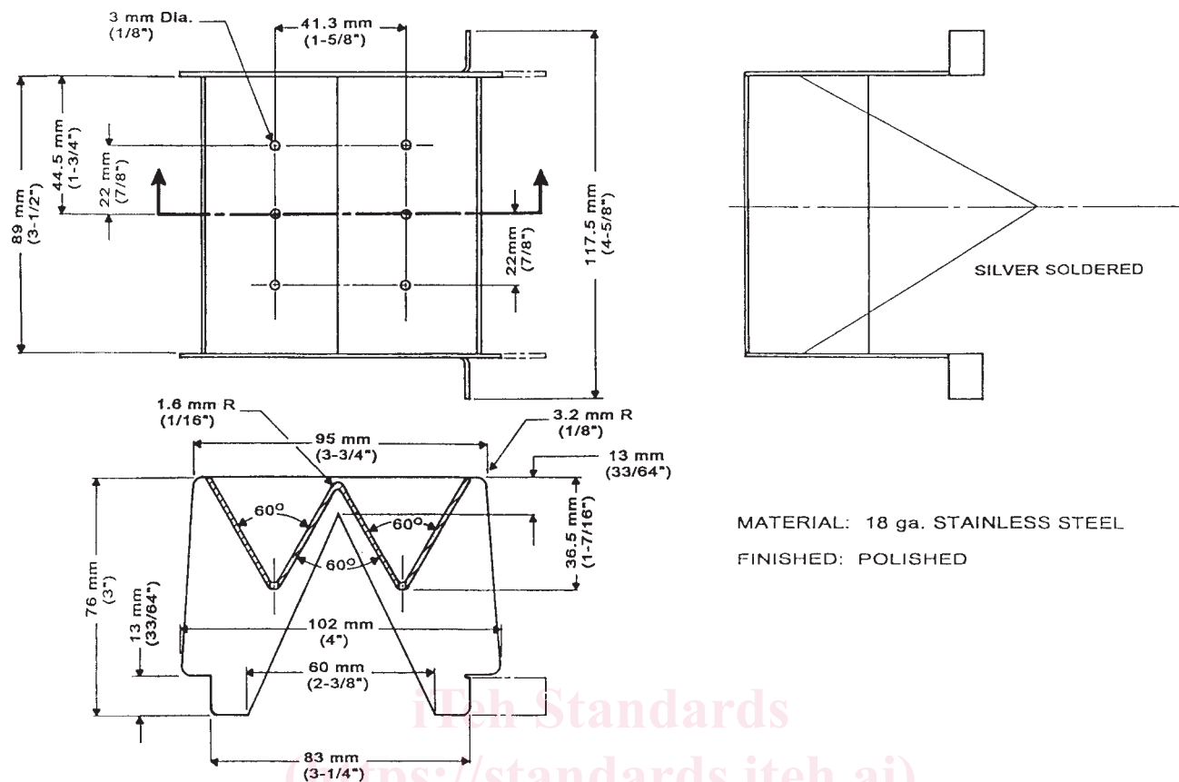
FIG. 1 Distribution Funnel
