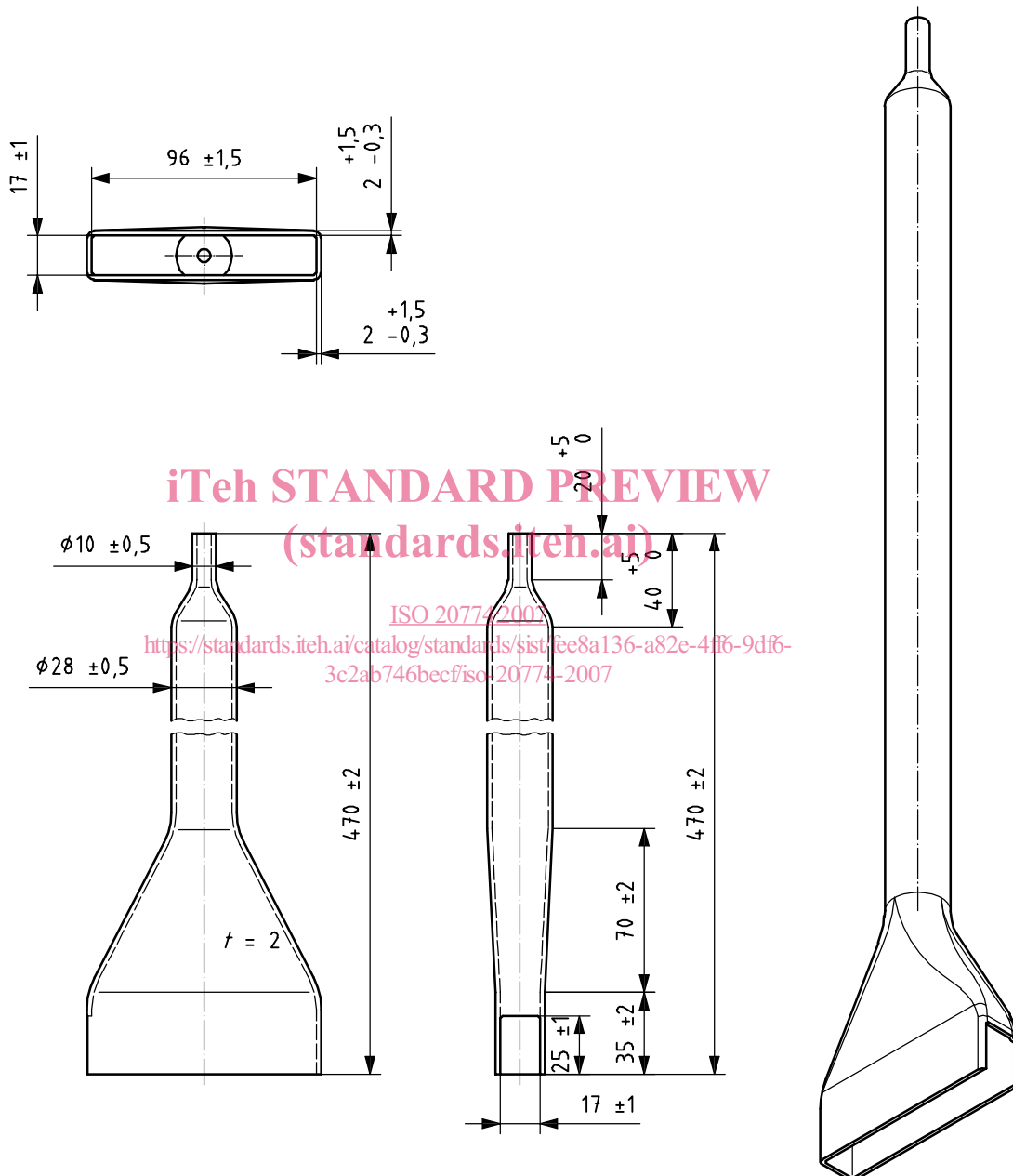
Figure 1 — Fishtail chimney dimensions
