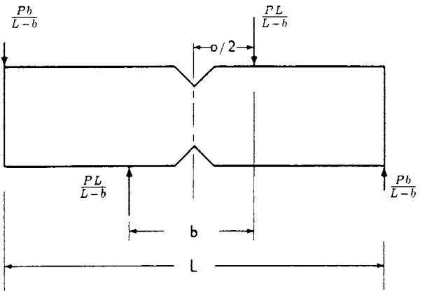
Force Diagram
