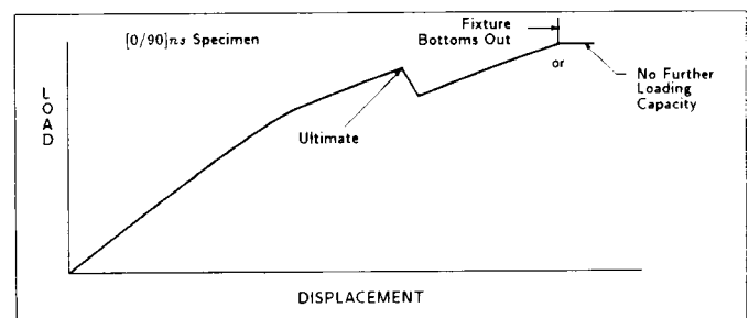
FIG. 5 Typical V-Notched Beam Load-Displacement Plots
