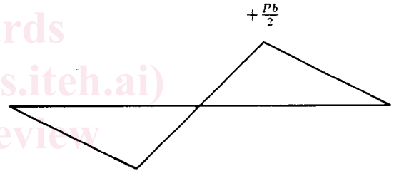
Shear Diagram
