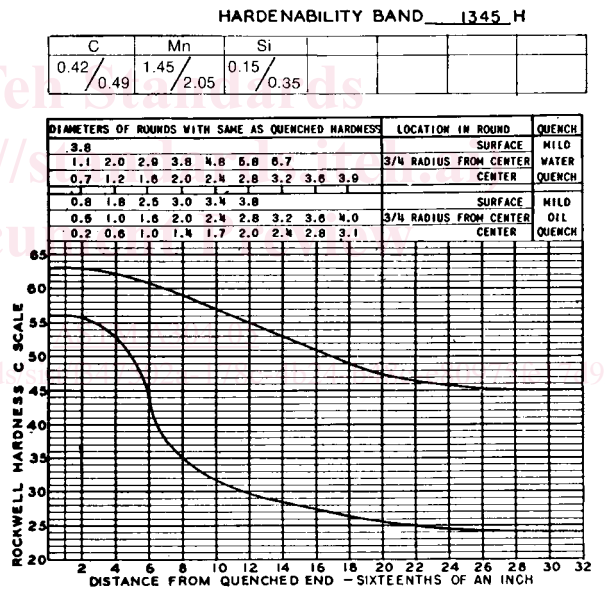
FIG. 5 Limits for Hardenability Band 1345 H
