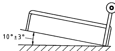
Figure 3 — Stability test in longitudinal direction
