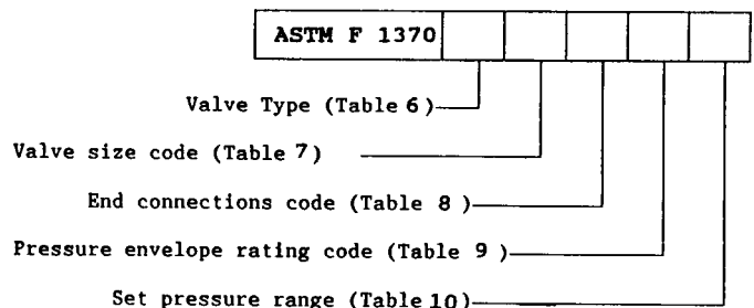
FIG. 1 Valve Coding System
