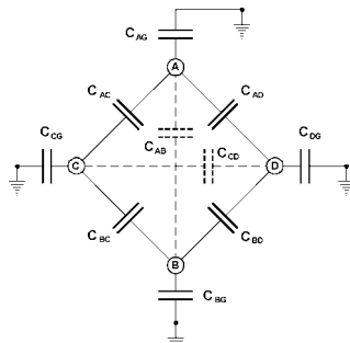
FIG. 2 Conductor Capacitances
