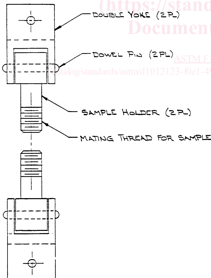
FIG. 1 Yoke and Dowel Pin Grips for Tensile Testing Porous Surfaces
