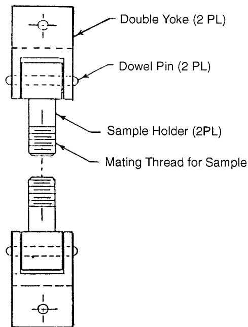
FIG. 2 Adaptor to Mate the Gripping Device to the Tensile Machine
