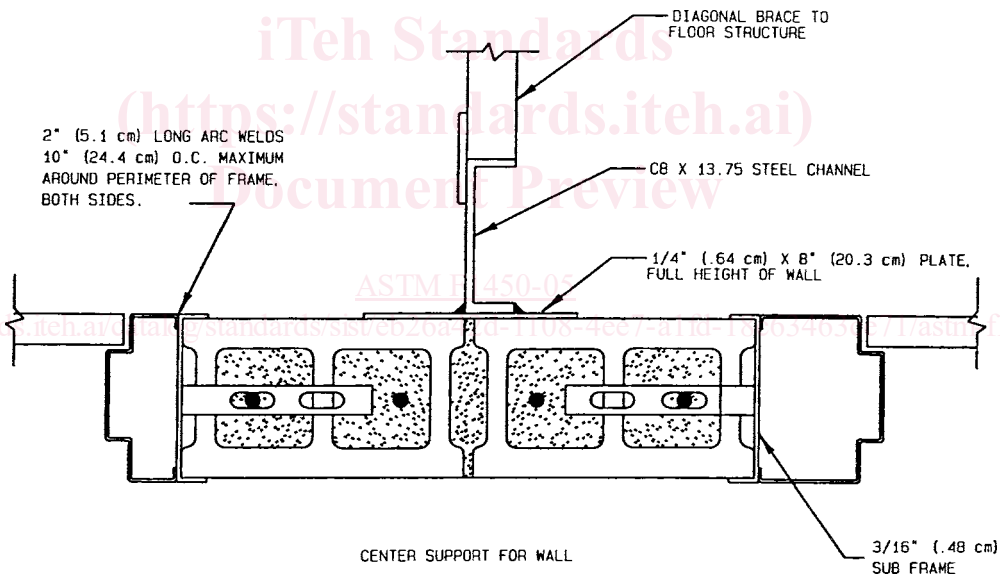
FIG. 4 Section C-C from Fig. 2
