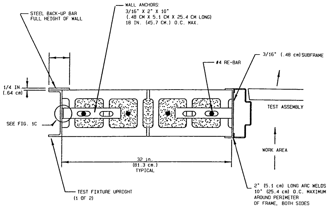
FIG. 3 Section B-B from Fig. 2
