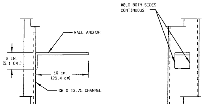
FIG. 5 Wall Anchor Welding Detention Hollow Metal Vision Systems
