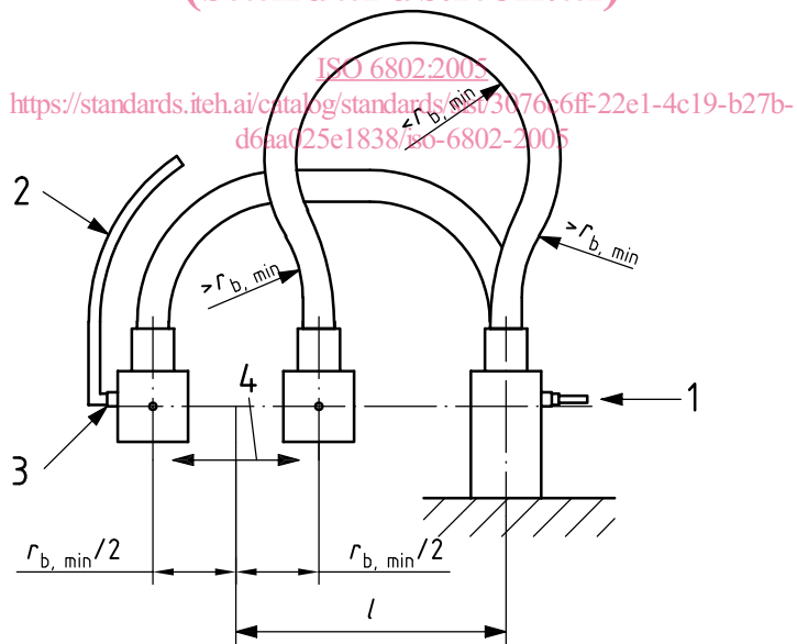
Figure 1 — Apparatus for hydraulic impulse test with flexing using a revolving manifold (standards.iteh.ai)
