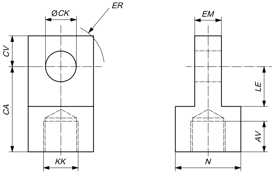
Figure 2 — AP4 — Rod eye, plain, female thread
