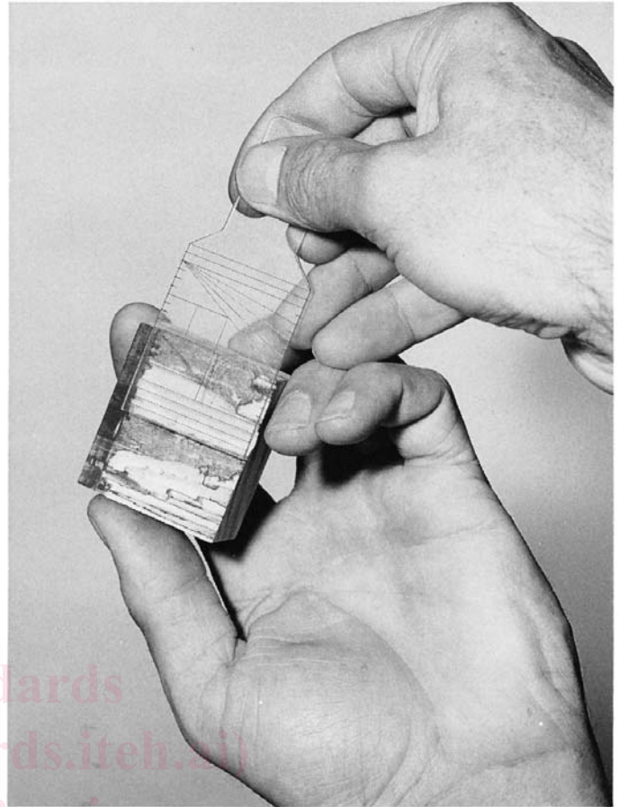
NOTE 1—In this case, a standard D905 shear block is shown.
