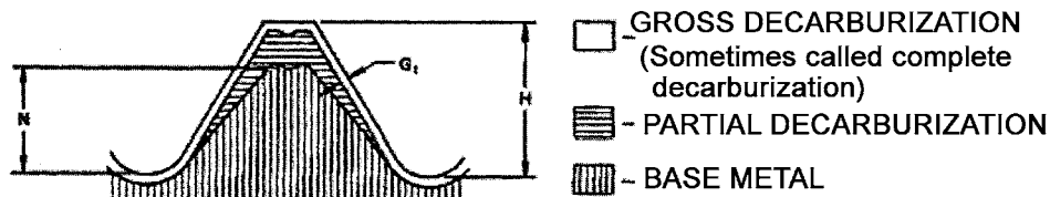
FIG. 1 Decarburization Zones
